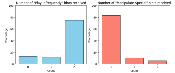
Figure 7: Distribution of specific hint types
