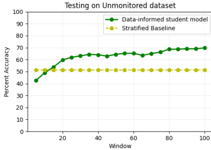
Figure 4: Evaluation of data-informed student model
