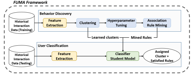
Figure 2: FUMA Framework
