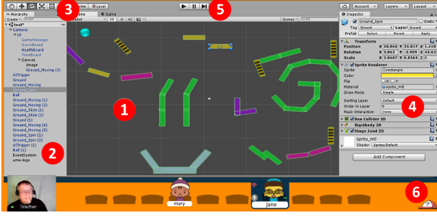
Figure 1: Unity-CT Environment
